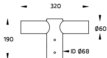
ATR-MOT-0004-XX Double head pole mount adapter 76mm pole diameter
