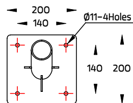
ATR-MOT-0003-XX Wall mount adapter
